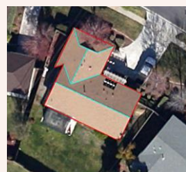
Significant lines detection
